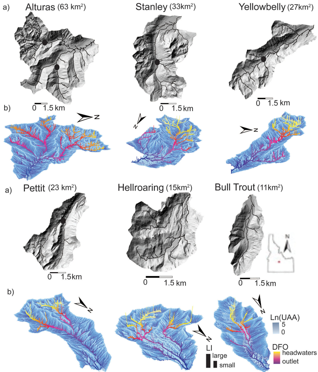
Figure 2. (a) Watersheds and stream networks displayed with hillshading to emphasize watershed shape and structure. Study location map at far right. (b) Upslope accumulated area superimposed on digital elevation models (DEMs) of each study watershed. Heights of bars along stream networks indicate magnitude of lateral inflow while bar colour indicates distance from watershed outlet. Points in the Alturas, Stanley, Yellowbelly, and Pettit watersheds indicate outlets of sub-watersheds used in analysis of the travel time function in watersheds of the same scale
