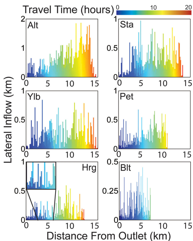
Figure 5. Distributions of lateral upland water contributions (bar height) and travel times (colour scale) over the range of stream network travel distances ( x -axis) in the Alt (Alturas), Blt (Bull Trout), Hrg (Hellroaring), Pet (Pettit), Sta (Stanley), and Ylb (Yellowbelly) watersheds. Multiple lateral inputs contributing at a given distance from the outlet can have different travel times as indicated by bars composed of multiple colours and demonstrated in the inset in the Hrg watershed. Note rescaled y -axes for Alt and Blt.
